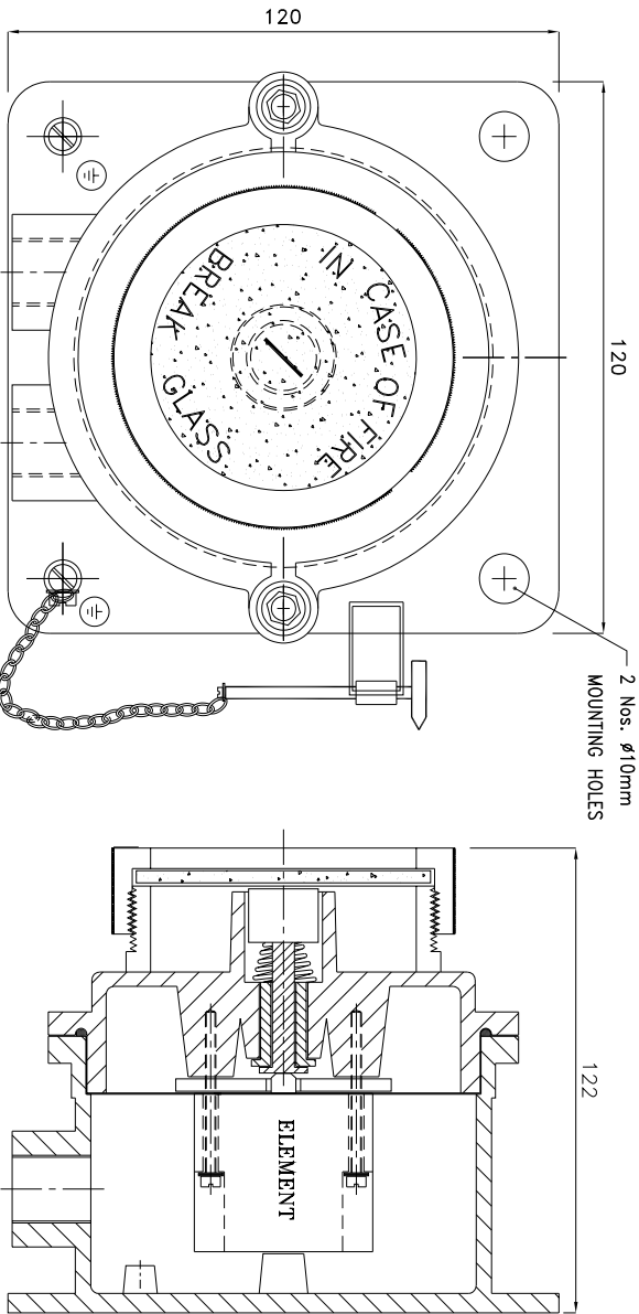
FRONT VIEW (BOTTOM SIDE) FRONT VIEW M.S. CHAIN WITH HAMMER
